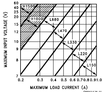
FIGURE 4. LM2575(HV)-5.0
